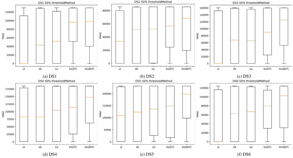
Fig. 22. Sensitivity analysis about prediction threshold method (C4) in middle testing phase.
