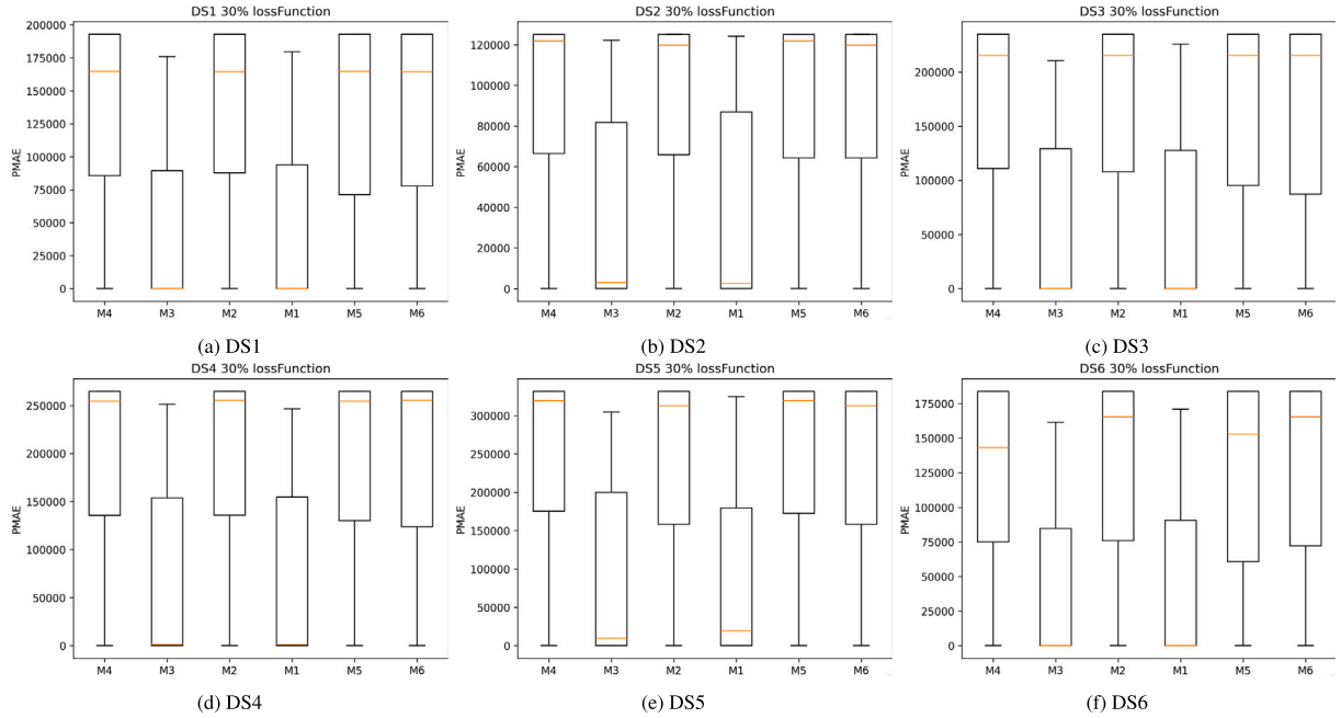
Fig. 18. Sensitivity analysis about prediction loss function (C3) in early testing phase.
