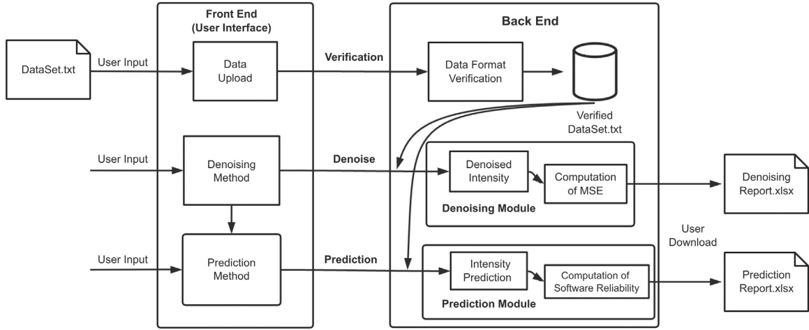
Fig. 1. System architecture.
