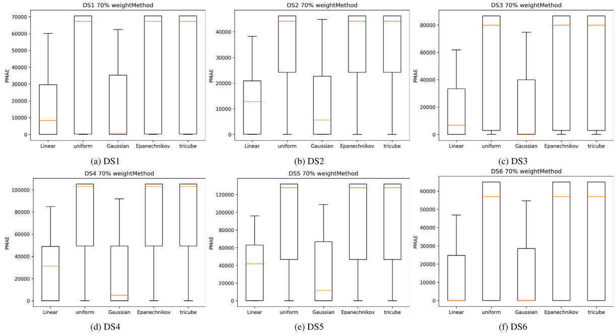
Fig. 17. Sensitivity analysis about prediction weight method (C2) in late testing phase.
