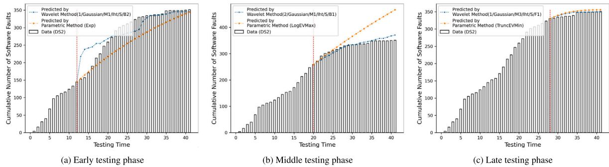
Fig. 7. Prediction behaviors of the cumulative number of software faults in DS2.
