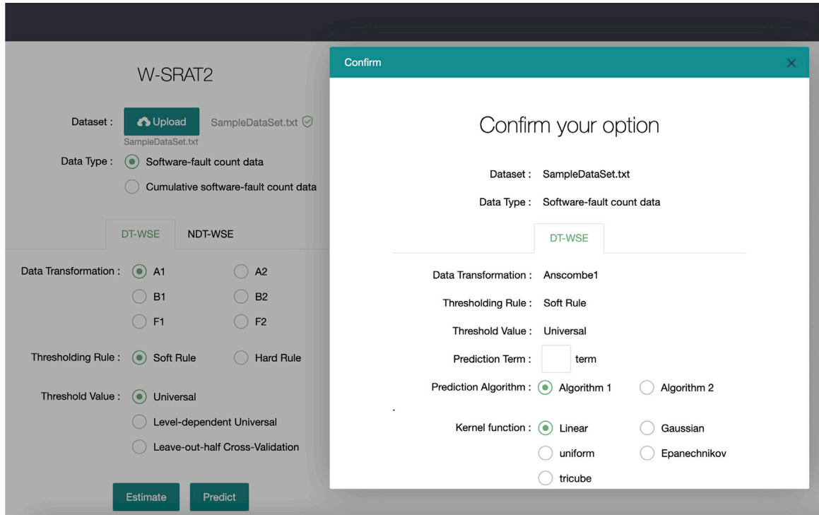
Fig. 2. Interface of W-SRAT2 (screenshot).
