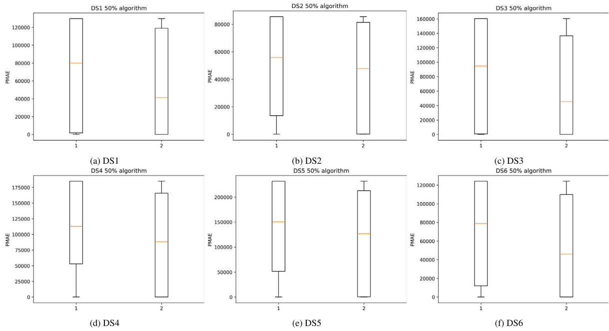
Fig. 13. Sensitivity analysis about prediction algorithm (C1) in middle testing phase.
