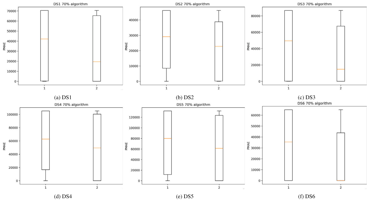
Fig. 14. Sensitivity analysis about prediction algorithm (C1) in late testing phase.
