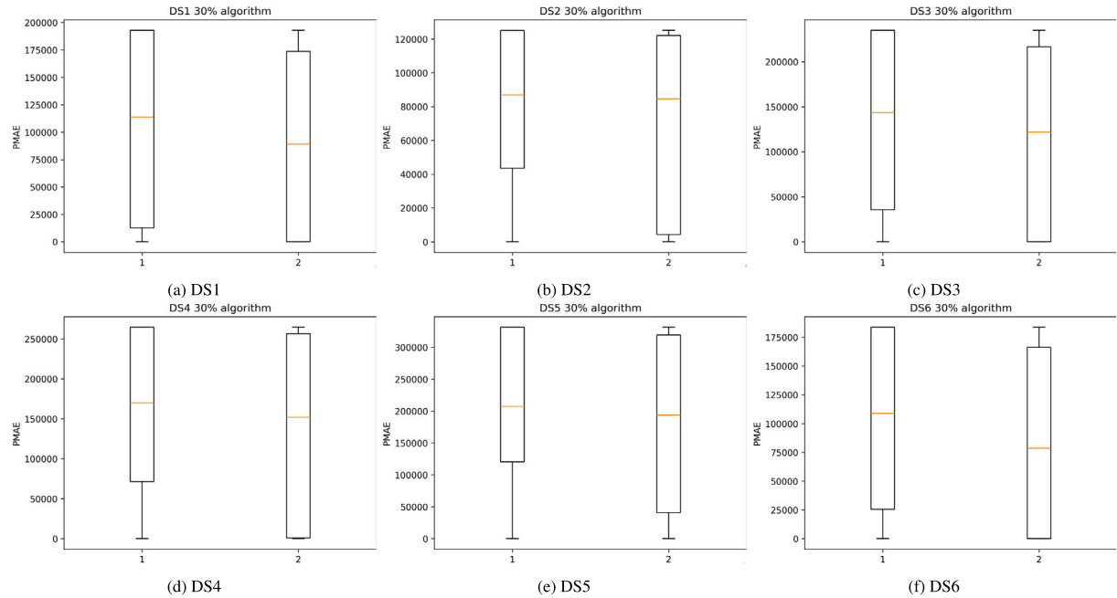
Fig. 12. Sensitivity analysis about prediction algorithm (C1) in early testing phase.
