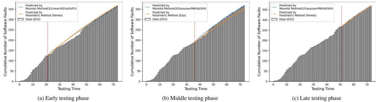
Fig. 8. Prediction behaviors of the cumulative number of software faults in DS3.
