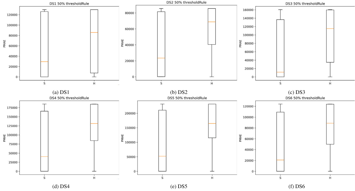
Fig. 25. Sensitivity analysis about prediction threshold rule (C5) in middle testing phase.
