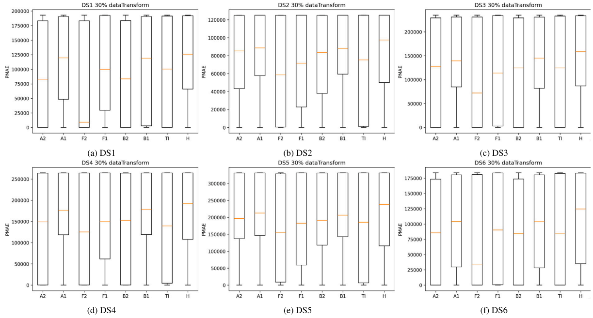
Fig. 27. Sensitivity analysis about prediction data transform (C6) in early testing phase.
